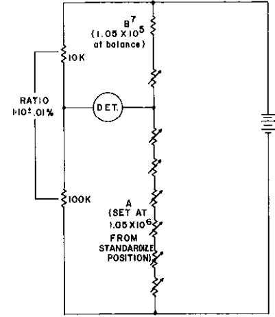
FIG. 7 BRIDGE IN CALIBRATE POSITION, MULTIPLIER AT 10^6
